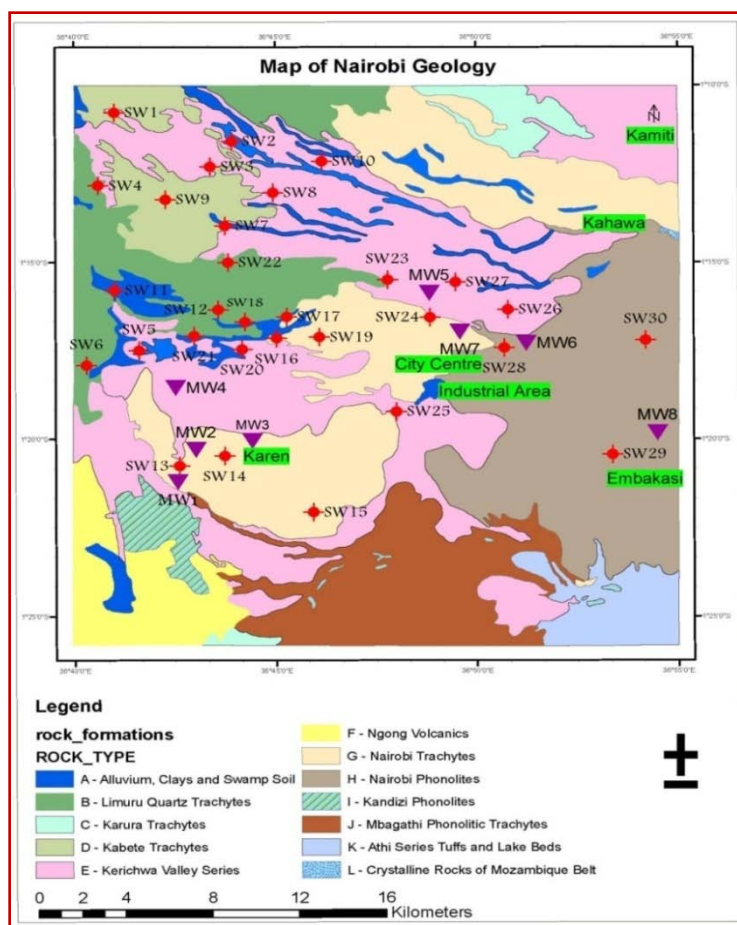
Figure 1 : Digitized geological map of Nairobi City (After Saggerson, 1991) showing study wells (SW) and monitoring wells (MW)
