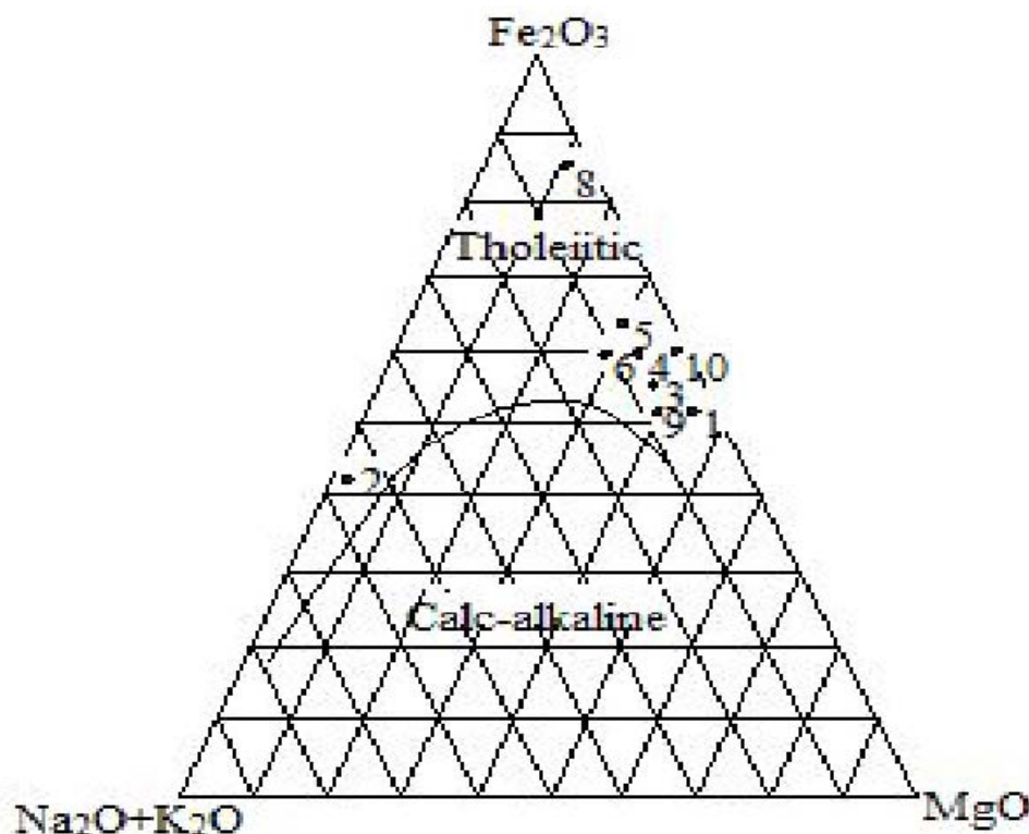
Figure 11 : Variation diagram showing the relationship of \text{Fe}_2\text{O}_3 with \text{Na}_2\text{O}_3 + \text{K}_2\text{O} and \text{MgO} (Method of Best and Christiansen, 2001)
