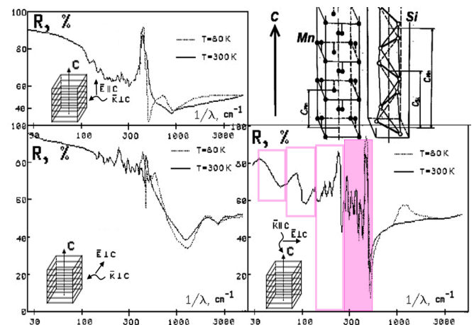
Figure 8. Crystal lattice of an incommensurate HMS quasicrystal (top, right) and the Giant Spatial Dispersion in its polarized IR reflection (the insets schematically indicate the direction of IR radiation propagation and its polarization relative to the concentration solitons in the HMS) [12].
